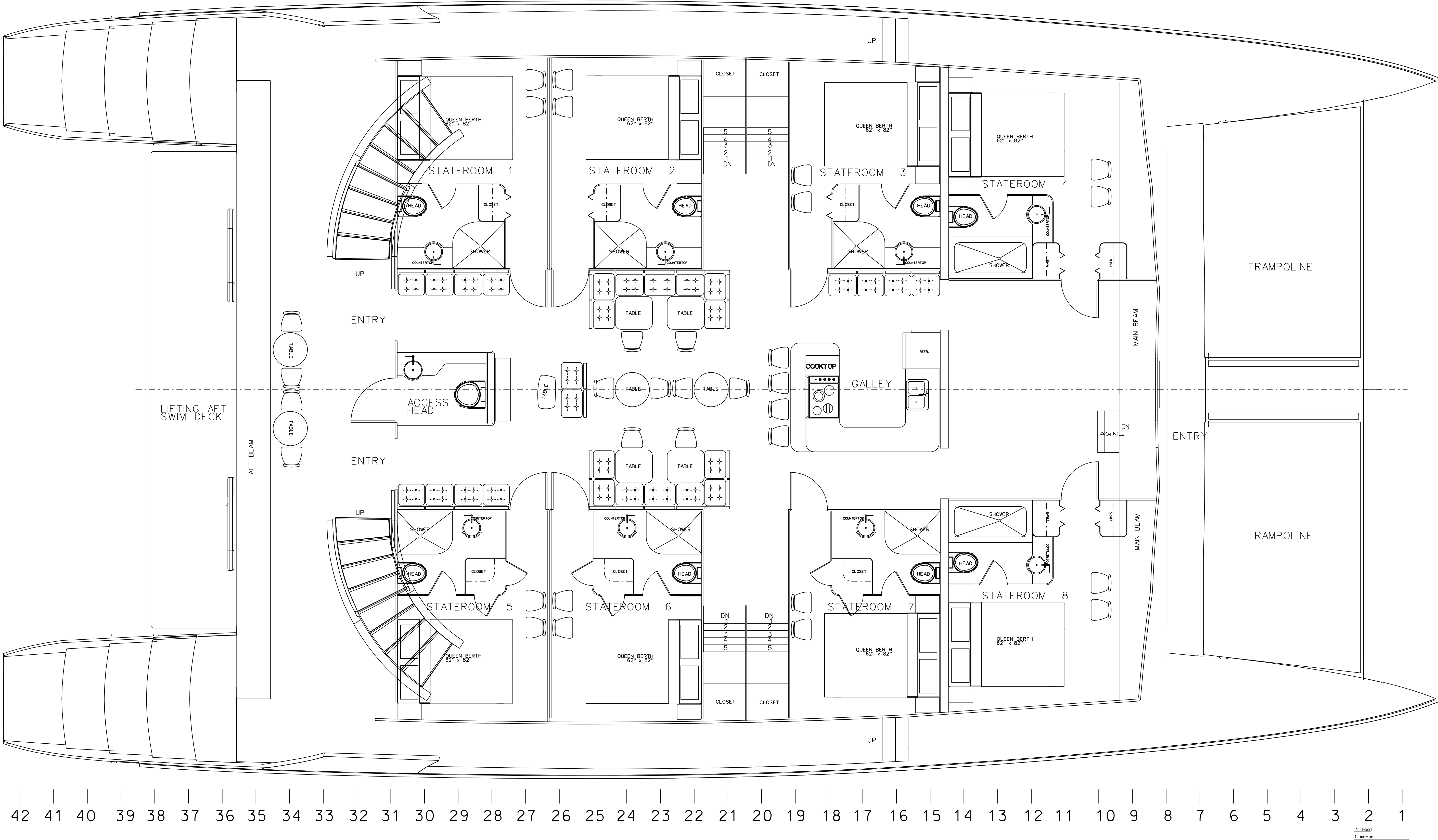
INTERIOR-MAIN LEVEL SCALE 3/8" = 1'-0"
