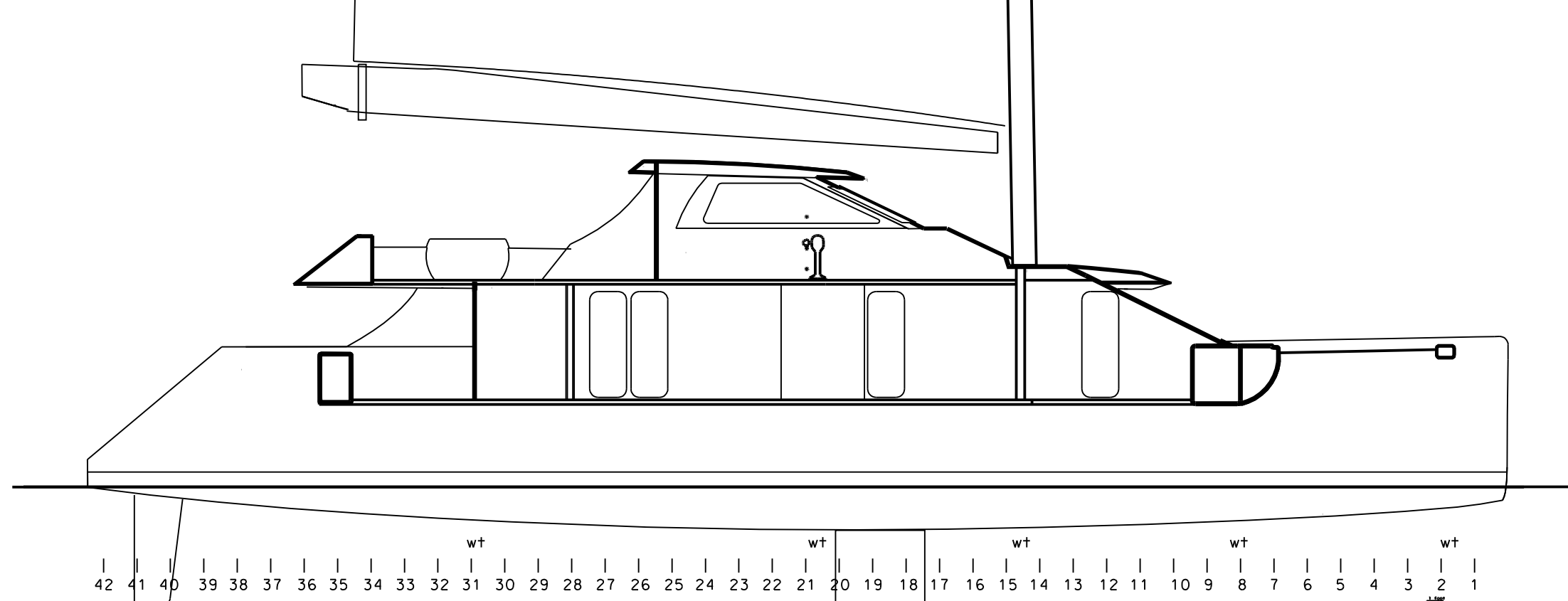
VESSEL CENTERLINE SECTION SCALE 1/2" = 1'-0"
