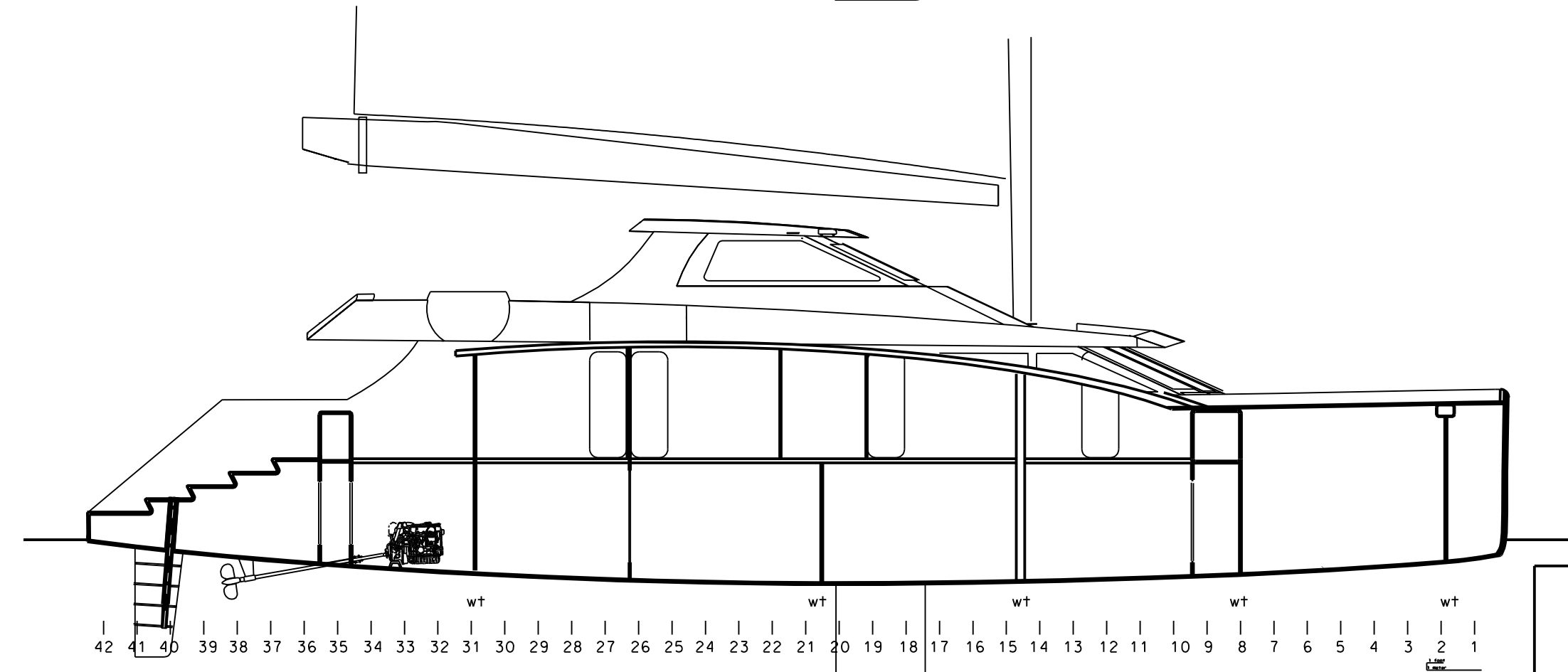
HULL CENTERLINE SECTION SCALE 1/2" = 1'-0"
